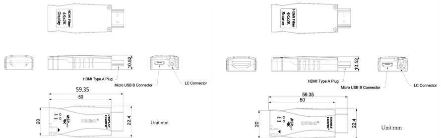
MSP 318-4 Transmitter
